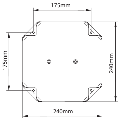
Base Plate
