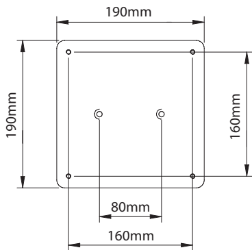
Speaker Platform
