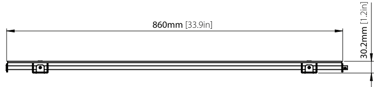
Wall Plate
