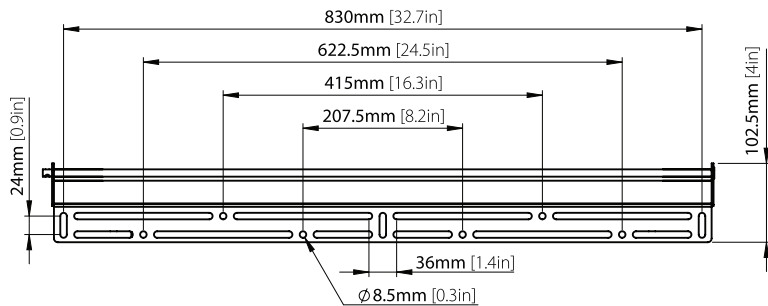
Wall Plate
