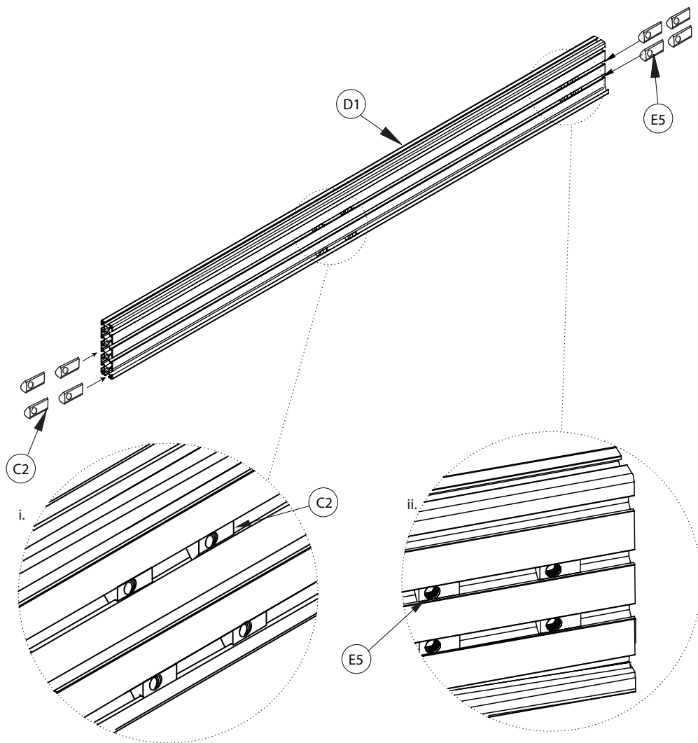
Angle Adjustment Connector Assembly
