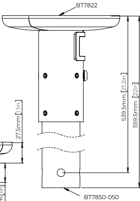
Pole Assembly Example
