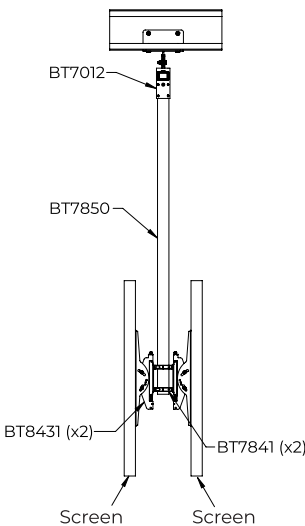
Back-to-Back Screen Pole Mounted
